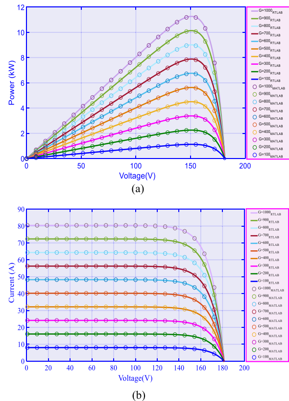
Fig. 15 Output characteristics of each photovoltaic array at 25 °C. a I - V curves and b P - V curves
