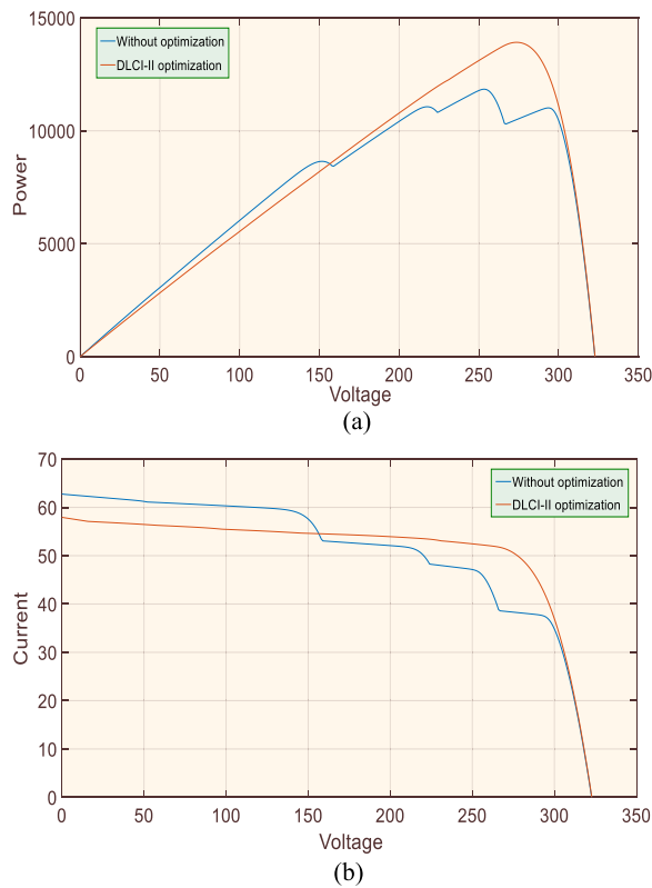
Fig. 12 Comparison result of PV arrays acquired by without optimization and DLCI-II in the 10th case of PSC. a P - V curves, and b I - V curves
