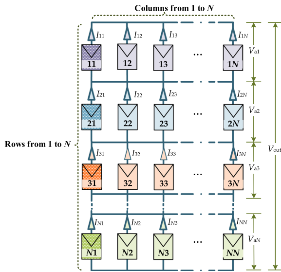
Fig. 2 N \times N TCT connected PV array
