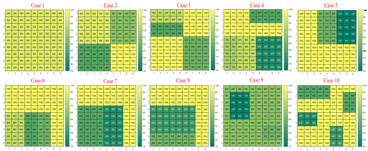
Fig. 7 The irradiation distribution of the 9 × 9 PV arrays in 10 cases of PSCs
