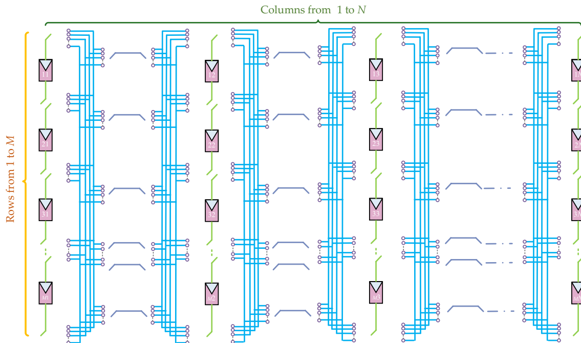
Fig. 4 Configuration of electrical switching arrangement
