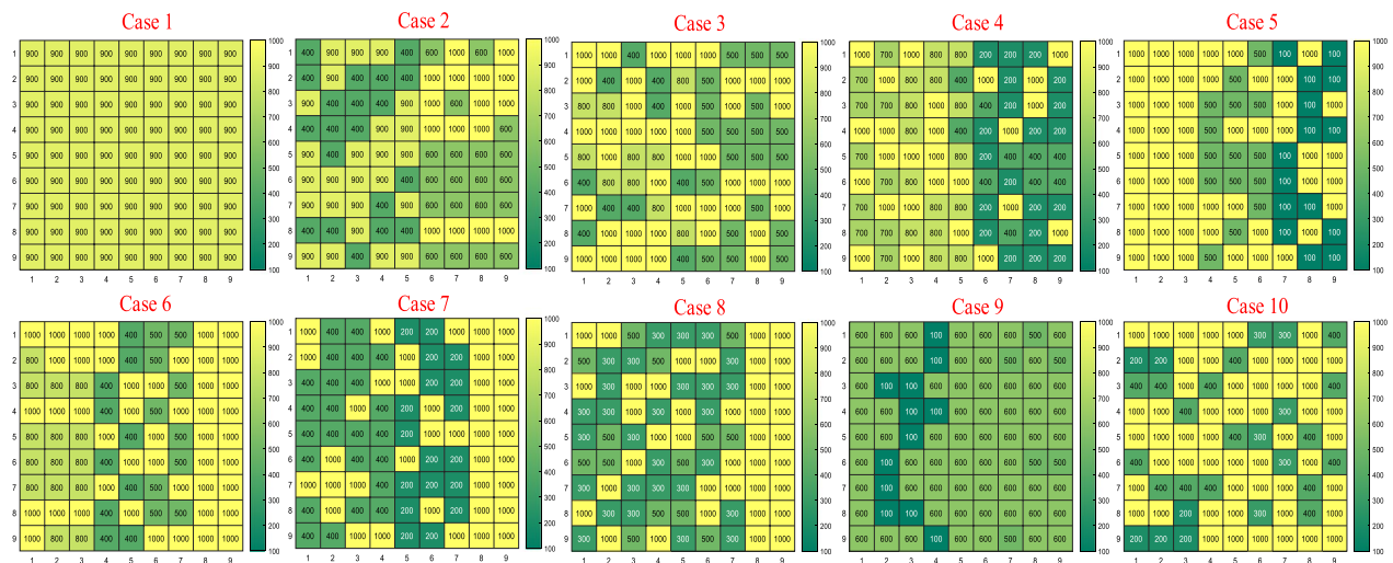
Fig. 11 The optimal solution of the 9×9 PV arrays reconfigured by DLCI-II with 10 cases of PSCs
