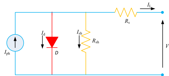
Fig. 1 Schematic diagram of a PV cell
