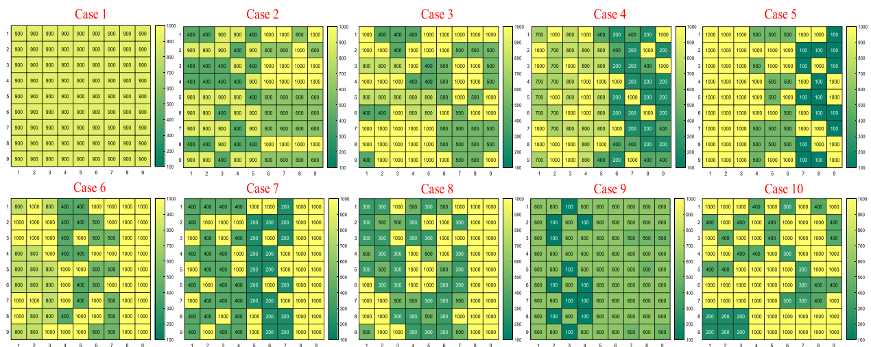
Fig. 9 The optimal solution of the 9 \times 9 PV arrays reconfigured by DLCI-I with 10 cases of PSCs
