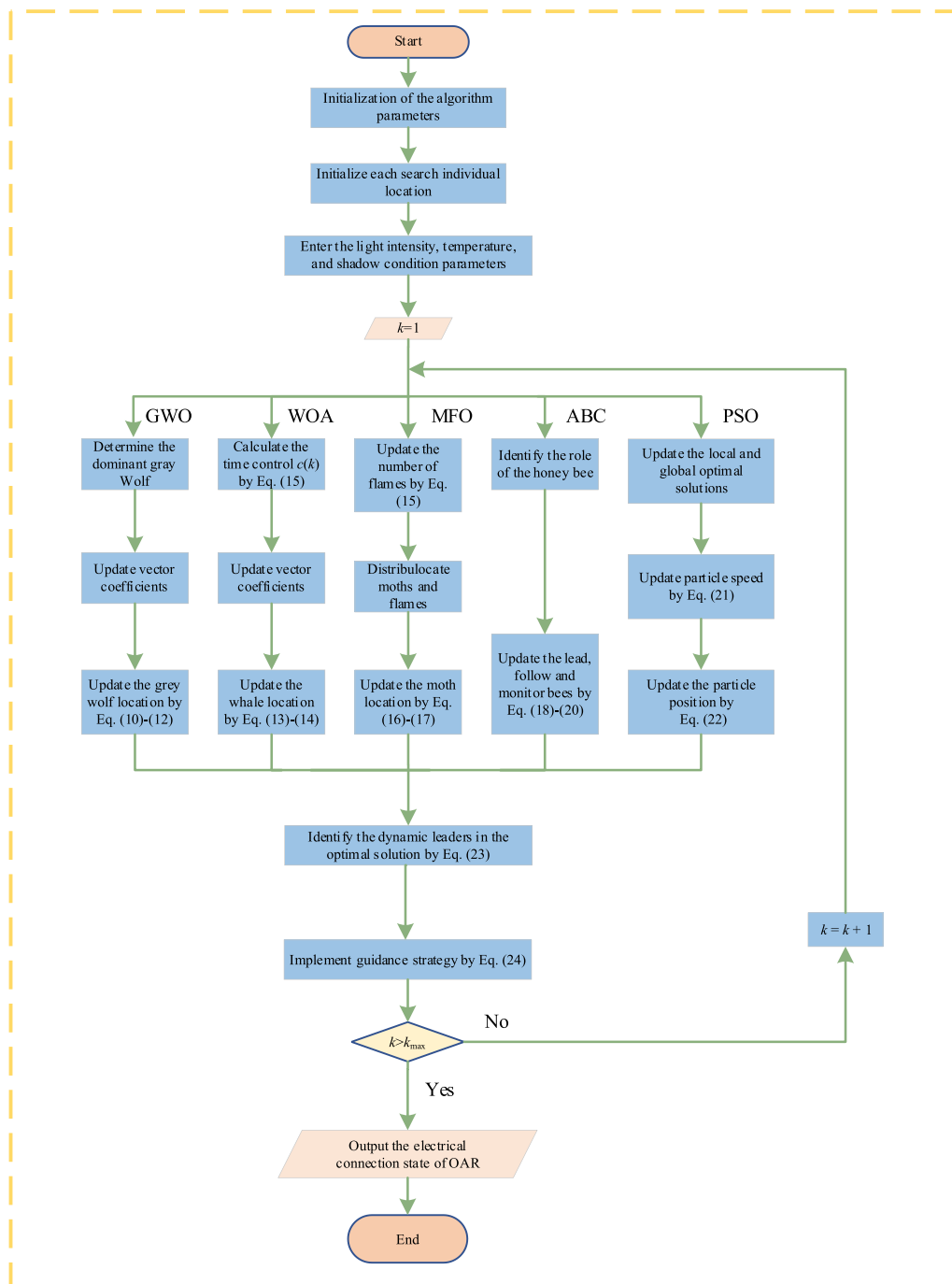
Fig. 6 Overall execution procedure of DLCI for PV array reconfiguration
