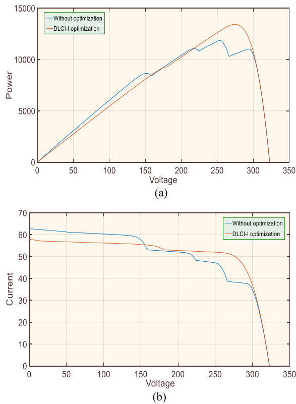
Fig. 10 Comparison result of PV arrays acquired without optimization and DLCI-I in the 10th case of PSC. a P - V curves, and b I - V curves
