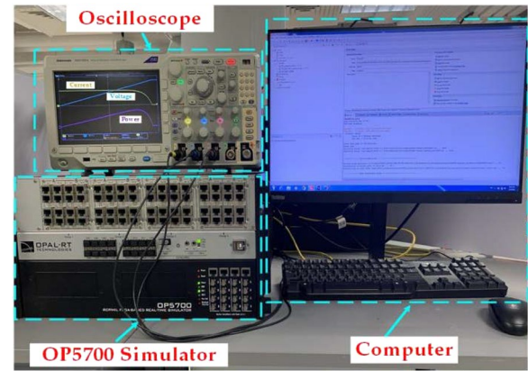
Fig. 14 Physical picture of hardware-in-the-loop test
