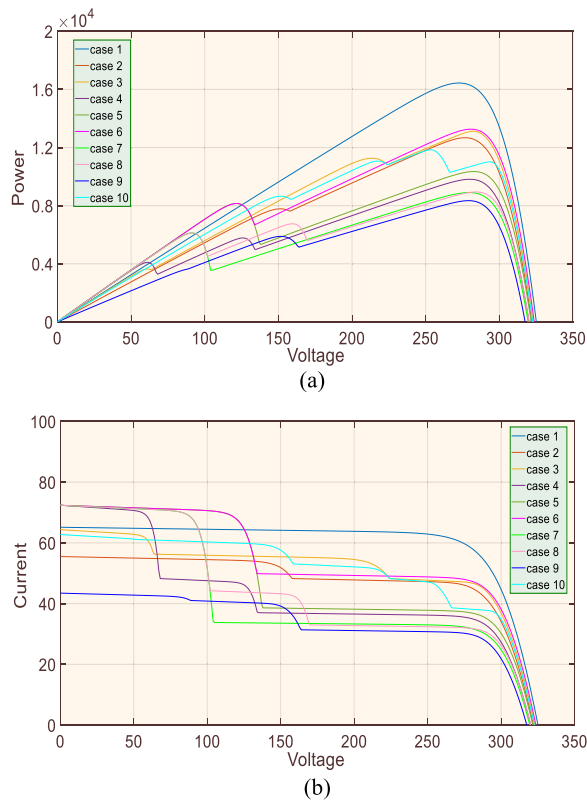
Fig. 8 Output results of the 9 \times 9 PV arrays in 10 cases of PSCs. a P - V curves, and b I - V curves
